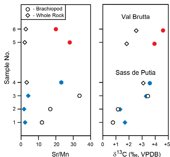
Fig. 5. Diagenetic screening of the brachiopod and whole rock material from the end Permian Bellerophon and Werfen Formations, northern Italy. Sr/Mn and \delta^{13}C values are used to discriminate between altered and preserved carbonates (cf. Brand and Veizer, 1980). Samples in solid colors were chosen for gas analysis based on preservation status (geochemical and microstructural evidence).
