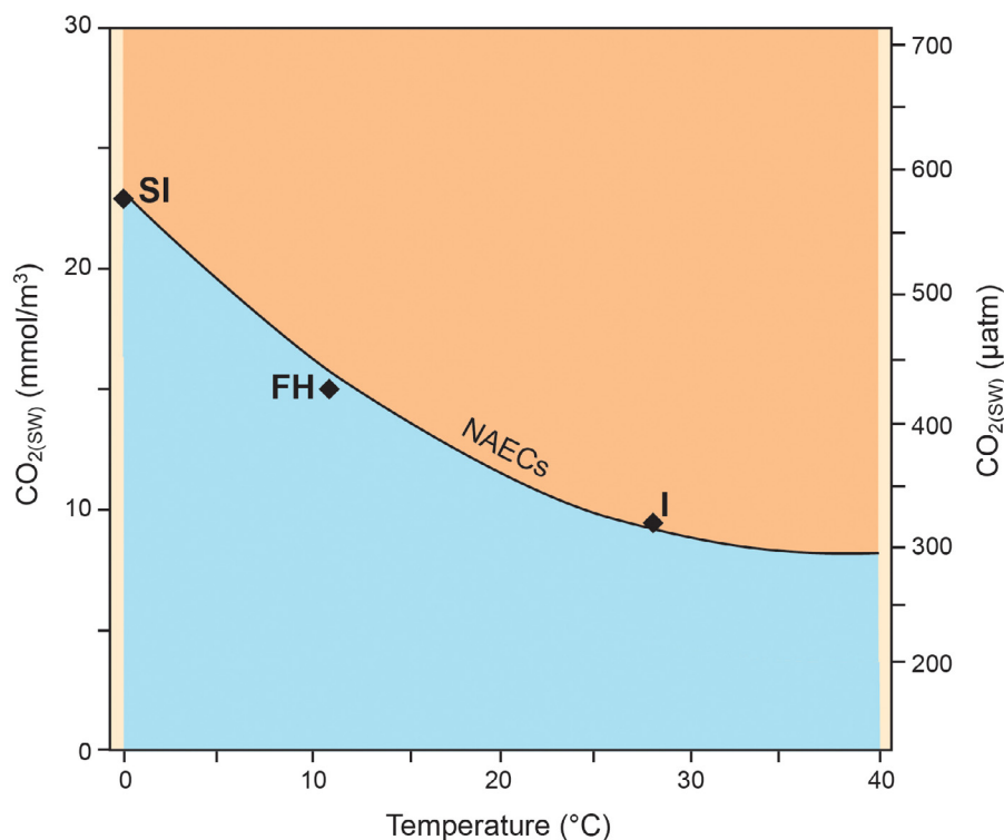
Fig. 2. Normal atmospheric equilibrium contents of gases in seawater and associated modern biogenic carbonates. The NAEC line represents equilibrium contents (dissolved) of carbon dioxide in modern seawater at temperatures ranging from 0 to 40 °C (Weiss, 1974). The SI, FH and I (black diamonds) are CO 2 contents of modern biogenic carbonates (brachiopods and coral) from Signy Island, Friday Harbor and Indonesia of shallow water depth (<100 m; Table 1).
