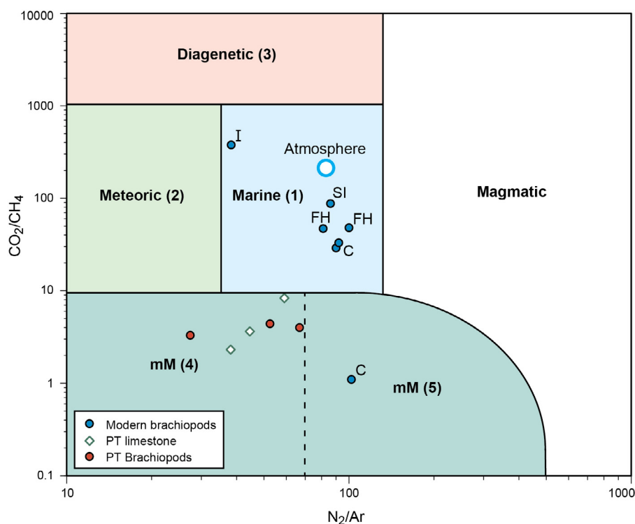
Fig. 6. Gas ratios of \text{CO}_2 , \text{CH}_4 , \text{N}_2 and Ar captured in vaulted pores of modern (C – Huinay, Chile; FH – Friday Harbor, USA; SI – Signy Island, Antarctica) and end Permian brachiopods and limestone of northeastern Italy (Table 2). Classification consists of five fields: Field 1 – Marine Carbonates: carbonates in gas equilibrium with seawater and atmosphere; Field 2 – Meteoric Carbonate: carbonates in gas equilibrium with freshwater system; Field 3 – Diagenesis: diagenetically altered material; Field 4 – modified Marine Carbonates: carbonates with gas ratios shifted due to changes in seawater chemistry; and Field 5 – modified Marine Carbonates: carbonates with gas ratios shifted due the change in seawater chemistry and bacterial carbonate reduction. Atmospheric \text{CO}_2/\text{CH}_4 – \text{N}_2/\text{Ar} ratio included for reference; general gas classification scheme and magmatic field are modified after Norman and Musgrave (1994).
