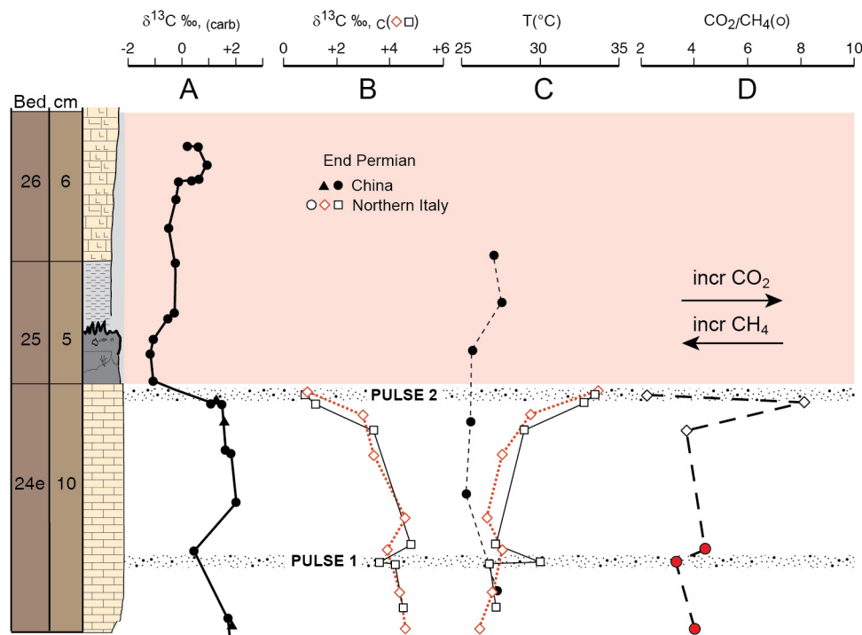
Fig. 7. Details of \delta^{13}\text{C} values, seawater temperatures, and gas content excursions at Meishan, China and northeastern Italy. Shaded field represents mass extinction period during the end Permian. Information: stratigraphy (Yin et al., 2001); column A: carbon isotope trends (China – Jin et al., 2000); column B: carbon isotope trend (northern Italy – Brand et al., 2012); column C: seawater temperatures (China – Joachimski et al., 2012; northern Italy – Brand et al., 2012); column D: changing \text{CO}_2/\text{CH}_4 gas ratios of this study. Pulses 1 and 2 correlate with trend in \delta^{13}\text{C} values from China and northern Italy, seawater temperatures and measured \text{CO}_2/\text{CH}_4 gas ratios. Gas symbols as in Fig. 6.
