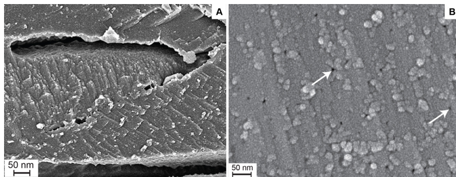
Fig. 4. High-resolution field-emission scanning electron micrographs of micro- and nano-structures within components of layers of modern brachiopods. (A) Close-up of gaps between fibers of the secondary layer in Notosaria nigricans created after hydrothermal removal of organic tissue. (B) Close-up and distribution of nanopores (arrows point to some pores) created by the hydrothermal removal of organic tissue in secondary layer fibers of Notosaria nigricans . Supplementary Figs. 1, 2 provide locality context.
